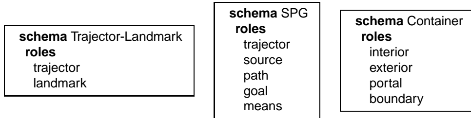
Figure 3: ECG formalism for schemas involved in the meaning of into . Keywords of the notation are shown in bold . The initial header line names the embodied schema being defined, followed by an indented roles block listing the schema role names.
