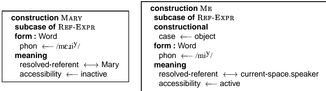
Figure 11: The MARY and ME constructions, both subcases of REF-EXPR , bind the Referent schema’s resolved-referent role to the Mary schema and the current speaker, respectively, and set different default levels of accessibility. The ME construction also constrains its case constructional feature.
