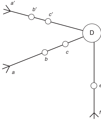
Fig. 3.4 Baginsky's (1871) diagram.
