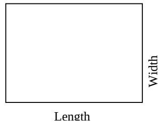
Figure 3.4: Two-dimensional container
