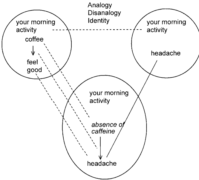
Figure 15.5. The caffeine headache network
